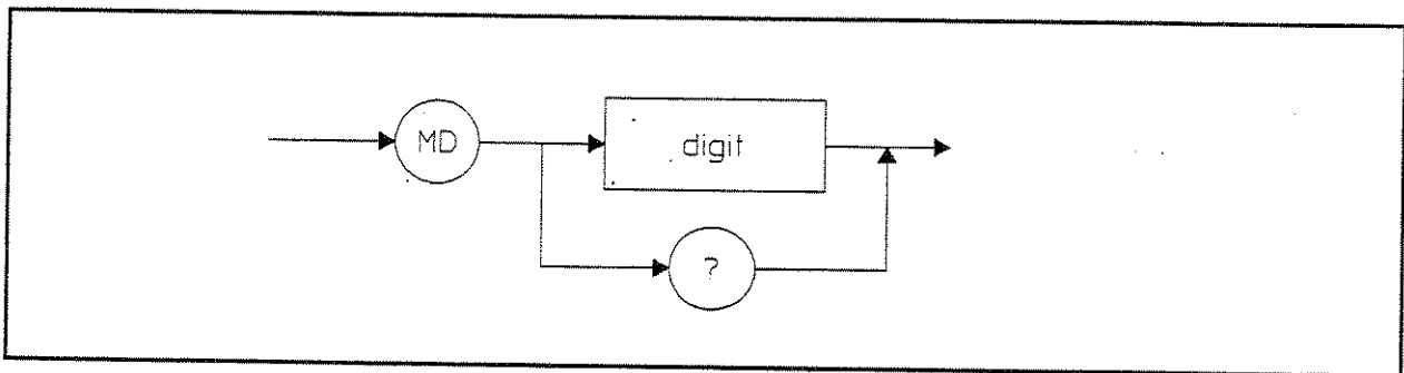
Figure 2-26. MD Syntax Diagram
